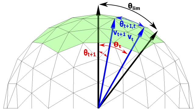
Figure 4: Tessellated hemisphere (dome) with two camera poses for the current ( t ) and next ( t + 1 ) state. The \theta_{lim} is the maximum allowed angle, \theta_t and \theta_{t+1} are the angles that camera viewpoints at states t , t + 1 make with the normal to the table and \theta_{t+1,t} is the angle between viewpoints v_t and v_{t+1} .
