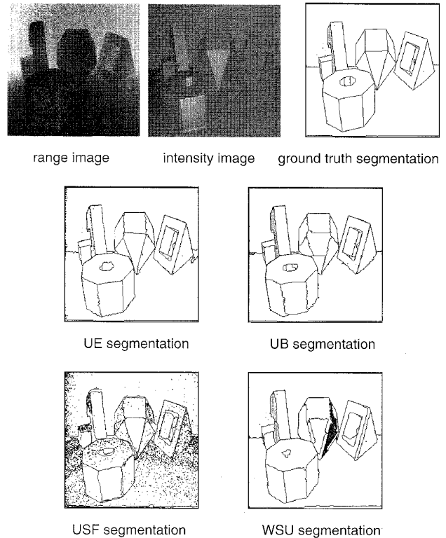
Fig. 14. Perceptron test image #26, which contains the largest GT region (2,124 pixels) that all four segmenters failed to correctly detect. The GT region's area is shaded gray in the segmentations. The "specks" were caused by the outlining of isolated noise or unlabeled pixels.
