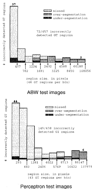
Fig. 12. Size distributions of GT regions incorrectly detected by UB segmenter.
