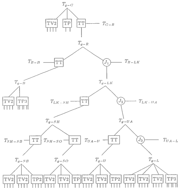
Figure 8: Robot Scene Geometric Reasoning Network
