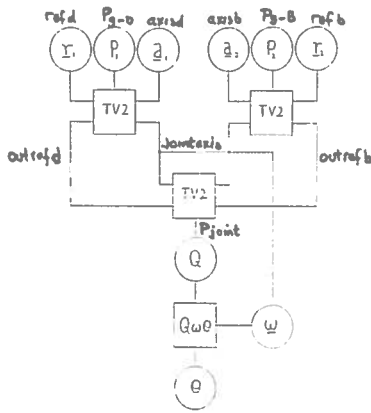
Figure 3: Revolute Joint Subnetwork
